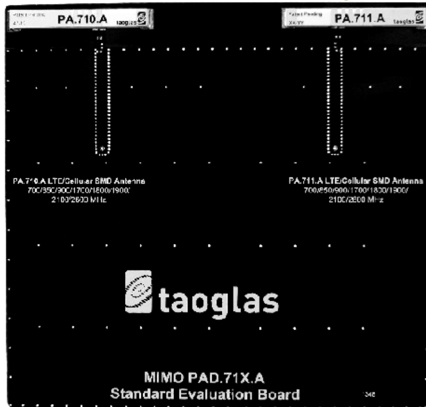
Figure 1. MIMO PAD.71X Standard Evaluation Board
