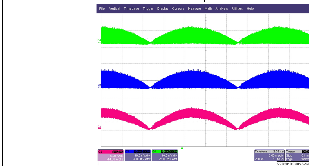
图 32. Inductor and Input Ripple Current at 85 V RMS at Peak of Line Voltage
