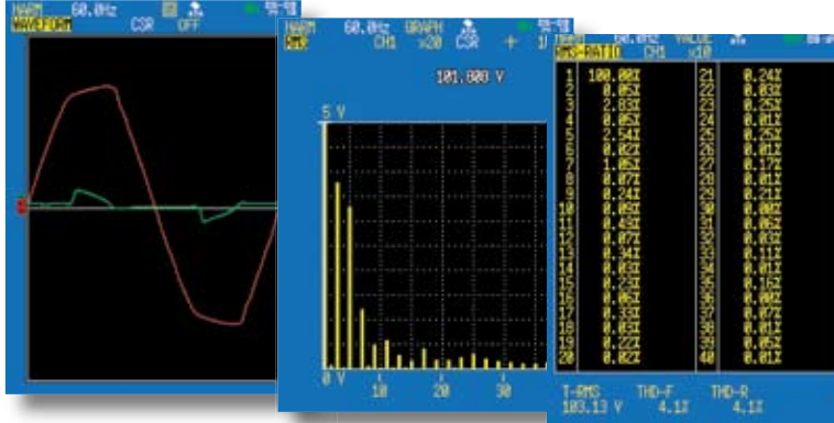
▲ Captured waveform (waveform display screen) ▲ RMS value of harmonic wave (bar graph) ▲ Content factor of harmonic wave (numeric data)
