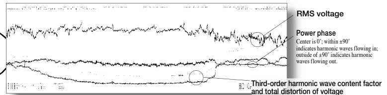
Harmonic wave time series recording example This graph shows that harmonic waves begin to decrease at 4:00 p.m., and then begin to increase at 6:30 a.m. the next morning.
