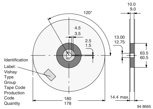
Figure 17. Reel dimensions - GS08
