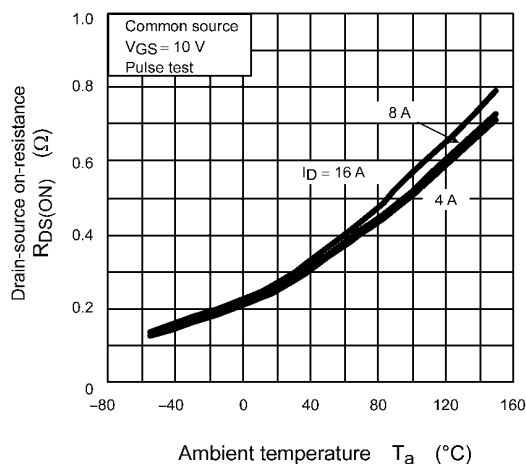
Fig. 8.7 R_{DS(ON)} - T_a
