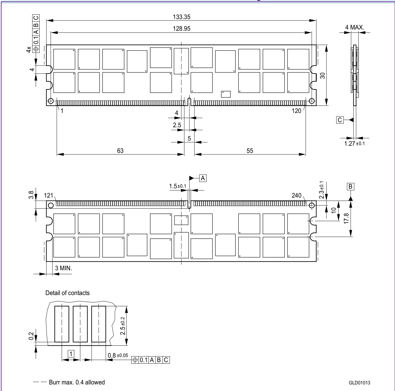
FIGURE 9 Package Outline Raw Card L L-DIM-240-40
