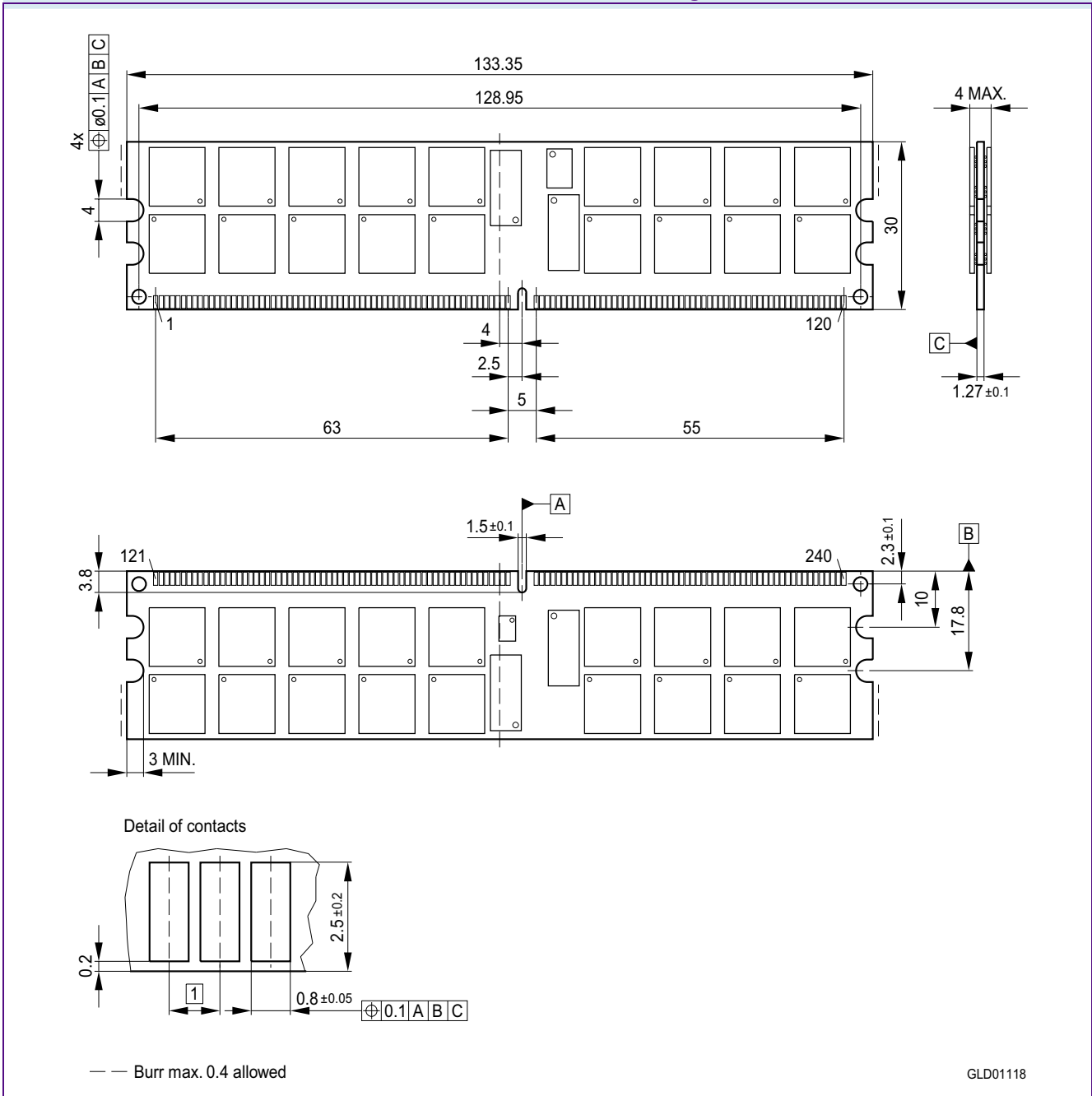
FIGURE 10 Package Outline Raw Card N – L-DIM-240-44
