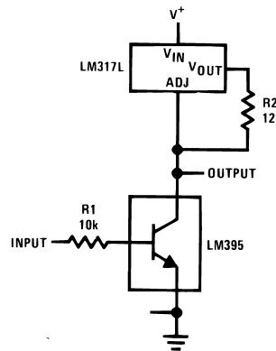
Figure 20. High Gain Amplifier
