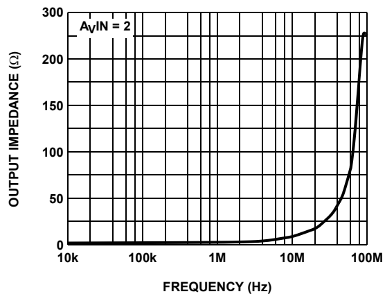
FIGURE 24. OUTPUT IMPEDANCE
