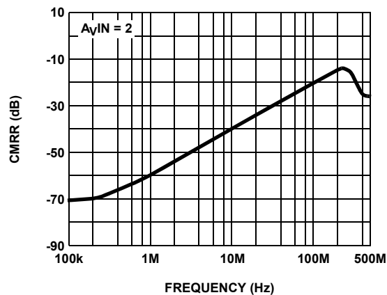
FIGURE 23. CMRR
