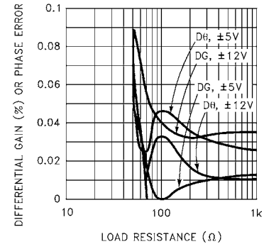
EL4430 Differential Gain and Phase Error vs R_L
