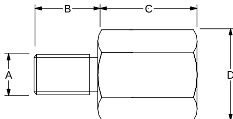
male fittings
