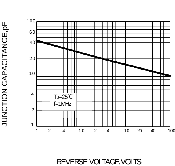
FIG.5-TYPICAL JUNCTION CAPACITANCE
