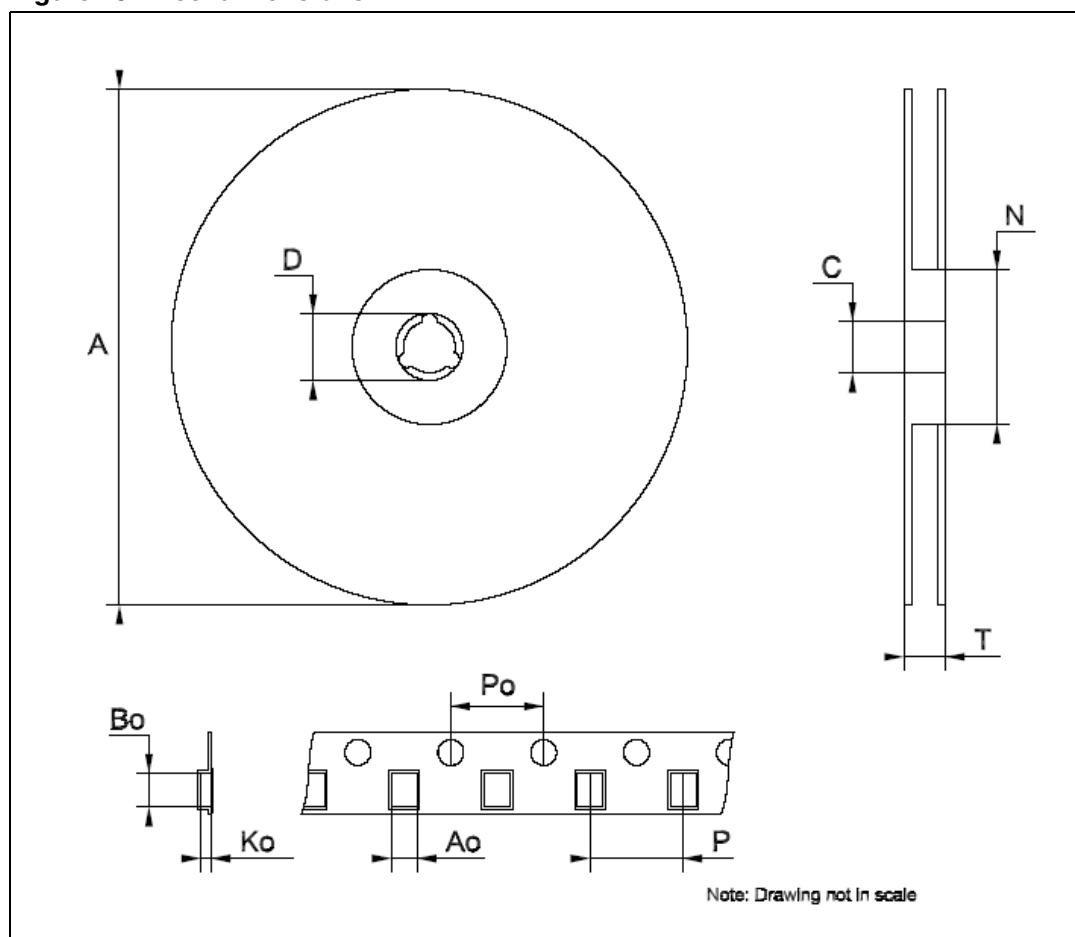
Figure 25. Reel dimensions
