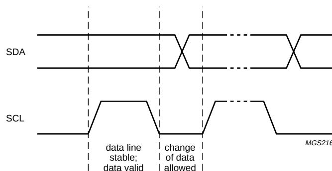
Fig.11 Bit transfer on the I 2 C-bus.
