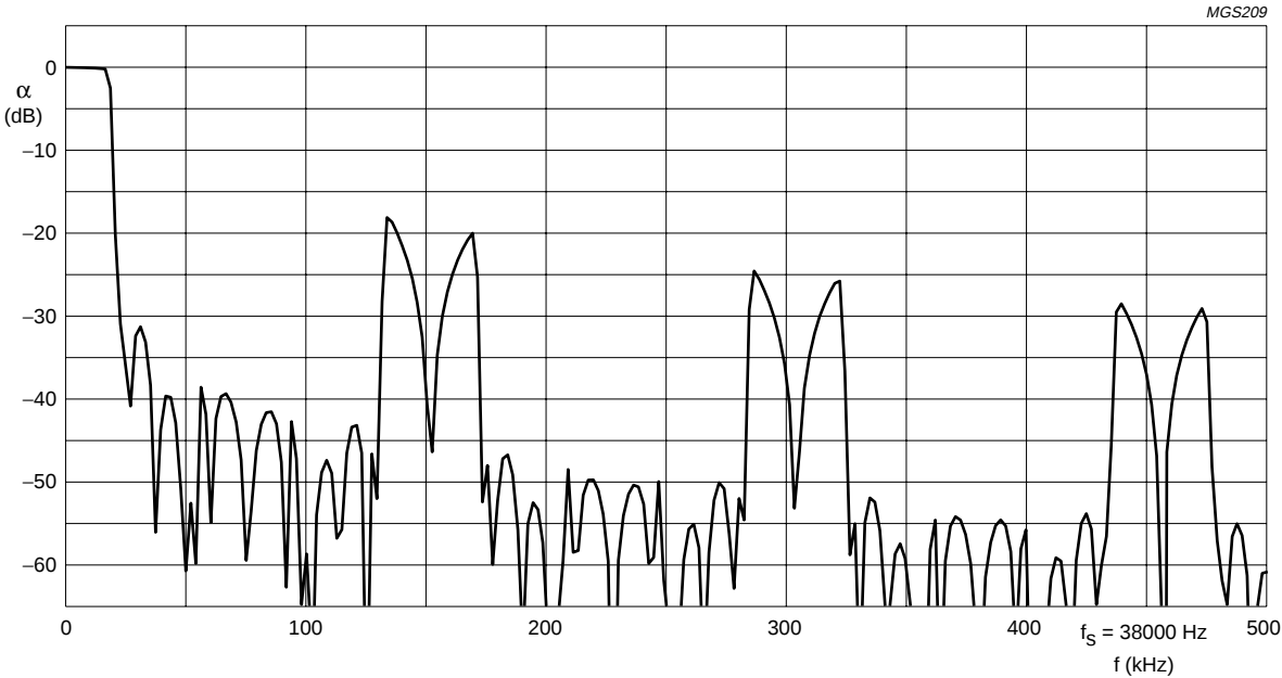
Fig.4 Overall frequency spectrum audio output.
