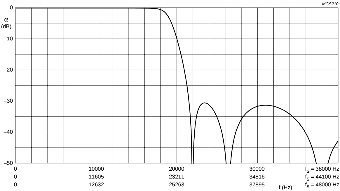
Fig.5 Detailed frequency spectrum audio output.
