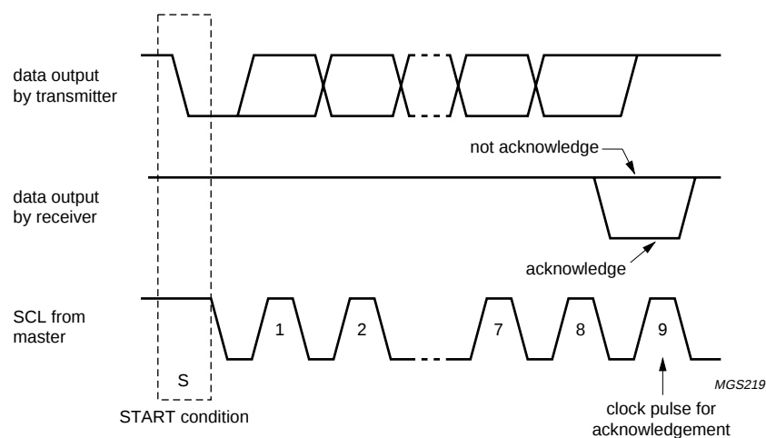
Fig.14 Acknowledge on the I 2 C-bus.
