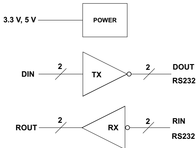
Simplified Diagram
