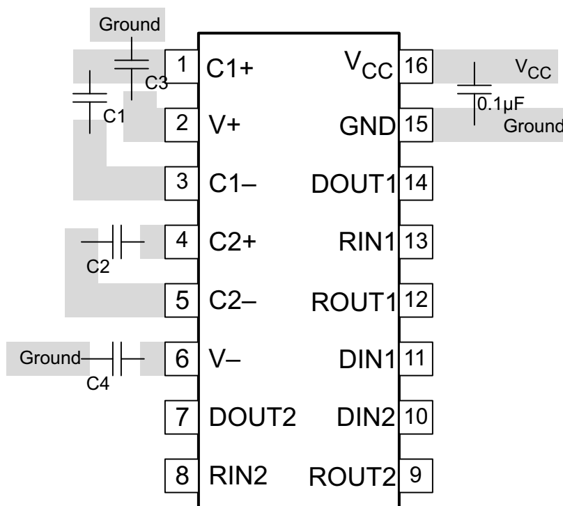
Figure 9. Layout Diagram
