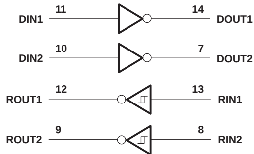
Figure 6. Logic Diagram
