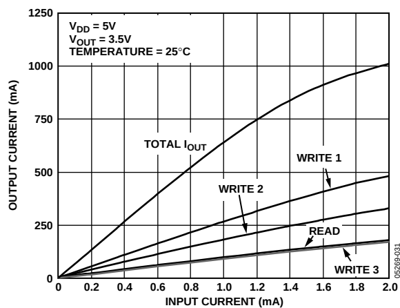
Figure 13. Output Current vs. Input Current for Each Channel, V_{OUT} = 3.5\text{ V}
