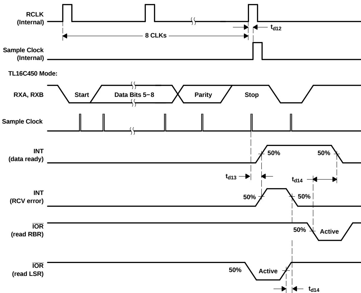
Figure 9. Receiver Timing Waveforms
