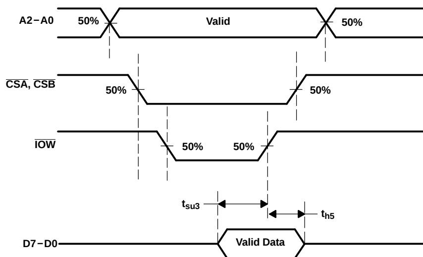
Figure 7. Write Cycle Timing Waveforms
