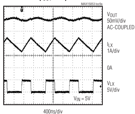
SWITCHING WAVEFORMS ( I_{OUT} = 2A )
