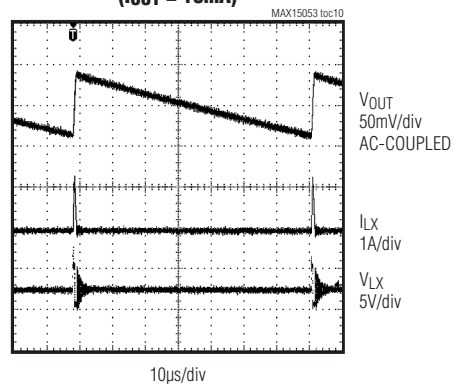
SWITCHING WAVEFORM IN SKIP MODE ( I_{OUT} = 10mA )
