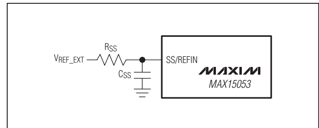
Figure 4. RC Network for External Reference at SS/REFIN
