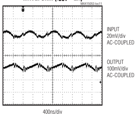
INPUT AND OUTPUT RIPPLE VOLTAGE WAVEFORM ( I_{OUT} = 2A )
