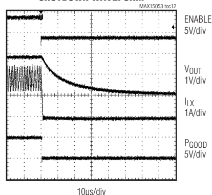
SHUTDOWN WAVEFORM
