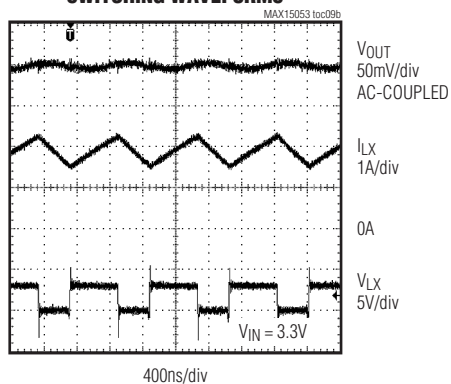
SWITCHING WAVEFORMS
