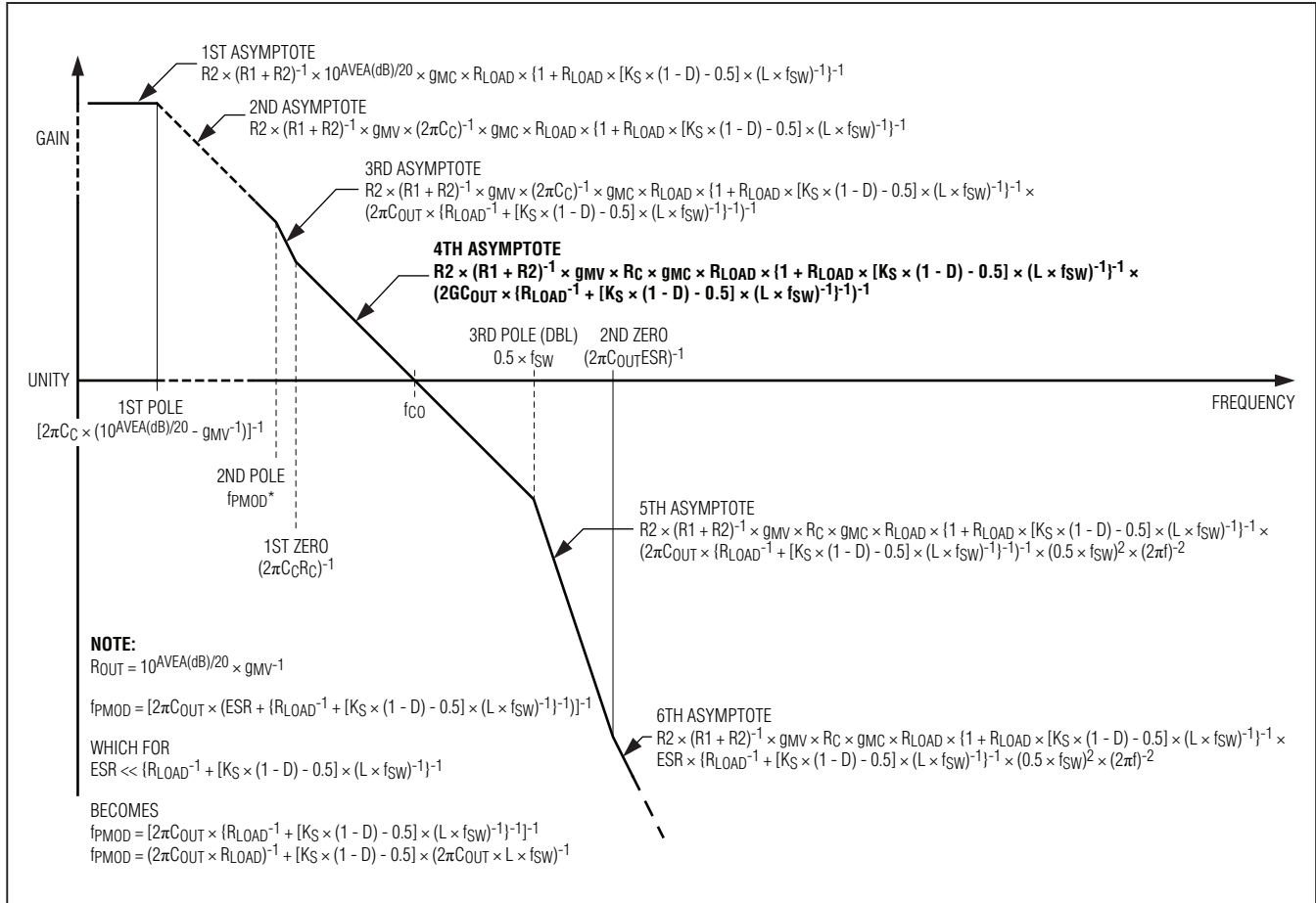
Figure 3. Asymptotic Loop Response of Current-Mode Regulator
