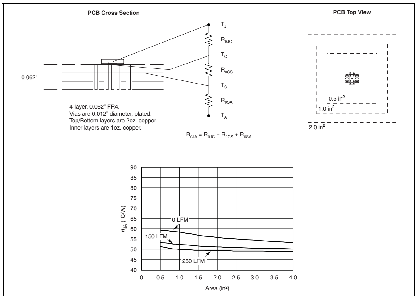
Figure 30. PCB Layout and Corresponding R_{\theta JA} Data, Vias Under Thermal Pad
