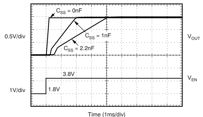
Figure 2. Turn-On Response
