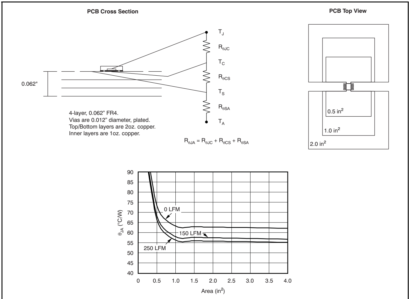
Figure 31. PCB Layout and Corresponding R_{\theta JA} Data, Top Layer Only
