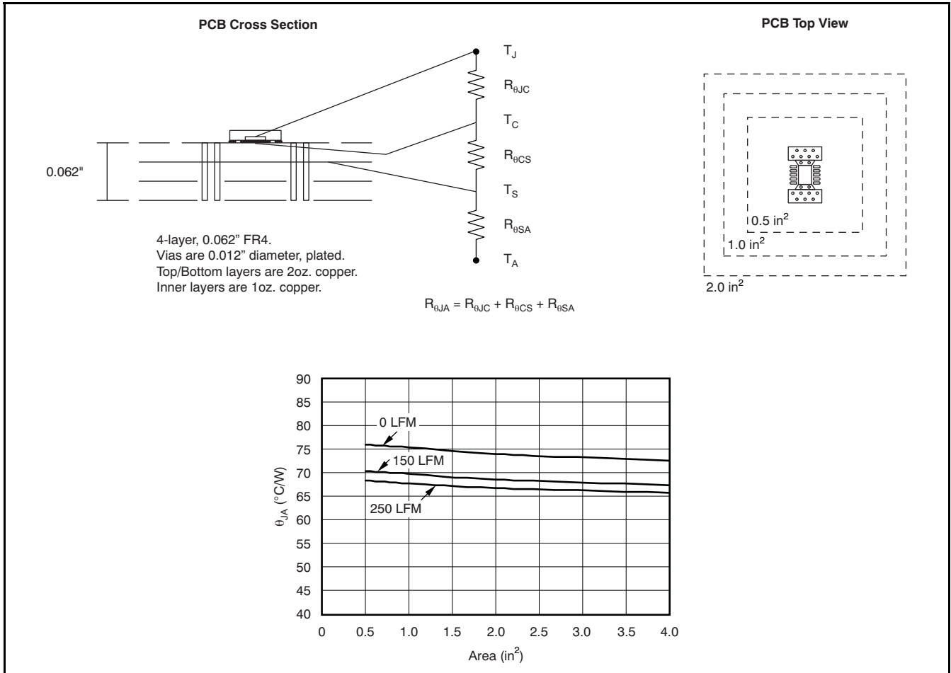
Figure 29. PCB Layout and Corresponding R_{\theta JA} Data, No Vias Under Thermal Pad
