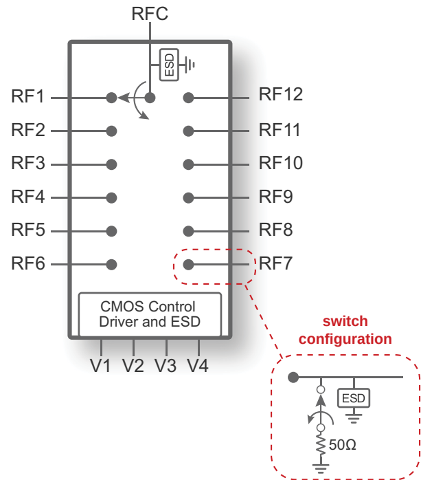
Figure 1 • PE42412 Functional Diagram
