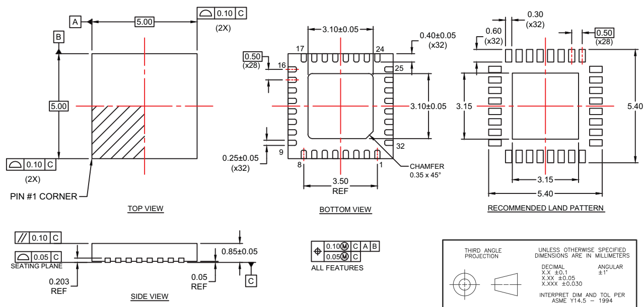
Figure 23 • Package Mechanical Drawing for 32-lead 5 × 5 × 0.85 mm QFN
