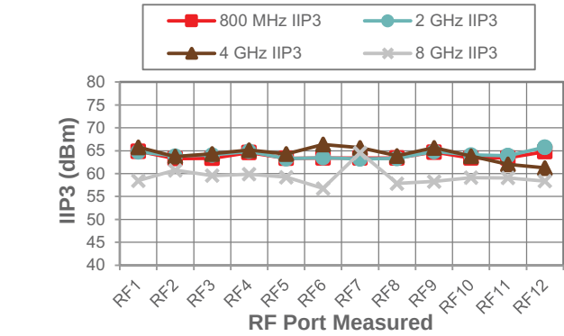
Figure 20 • IIP3 vs. RF Port Measured
