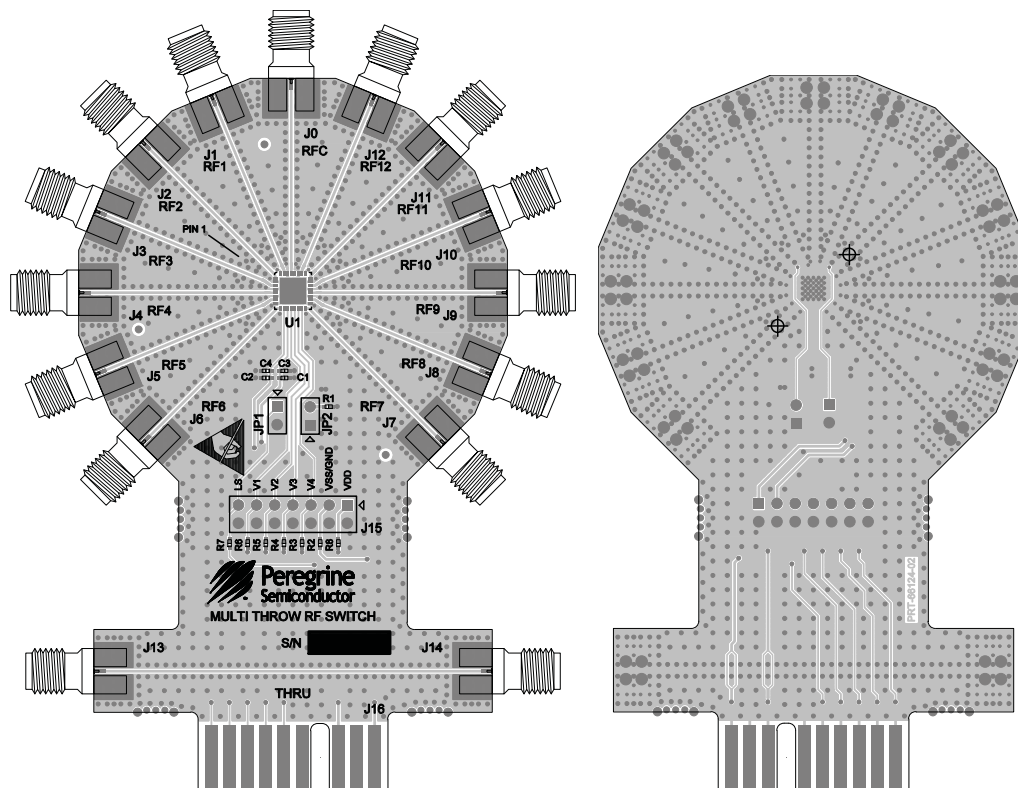
Figure 21 • Evaluation Board Layout for PE42412
