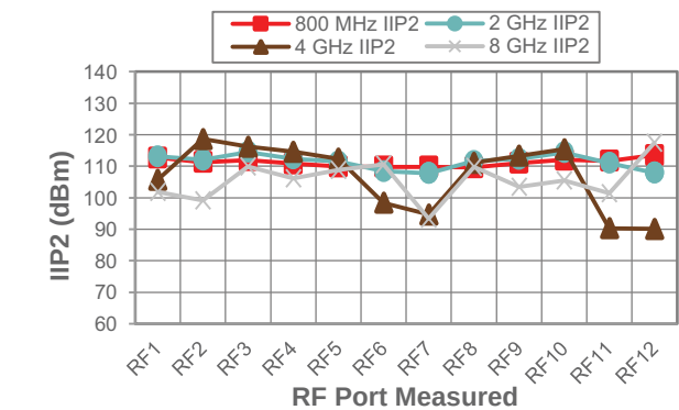
Figure 19 • IIP2 vs. RF Port Measured
