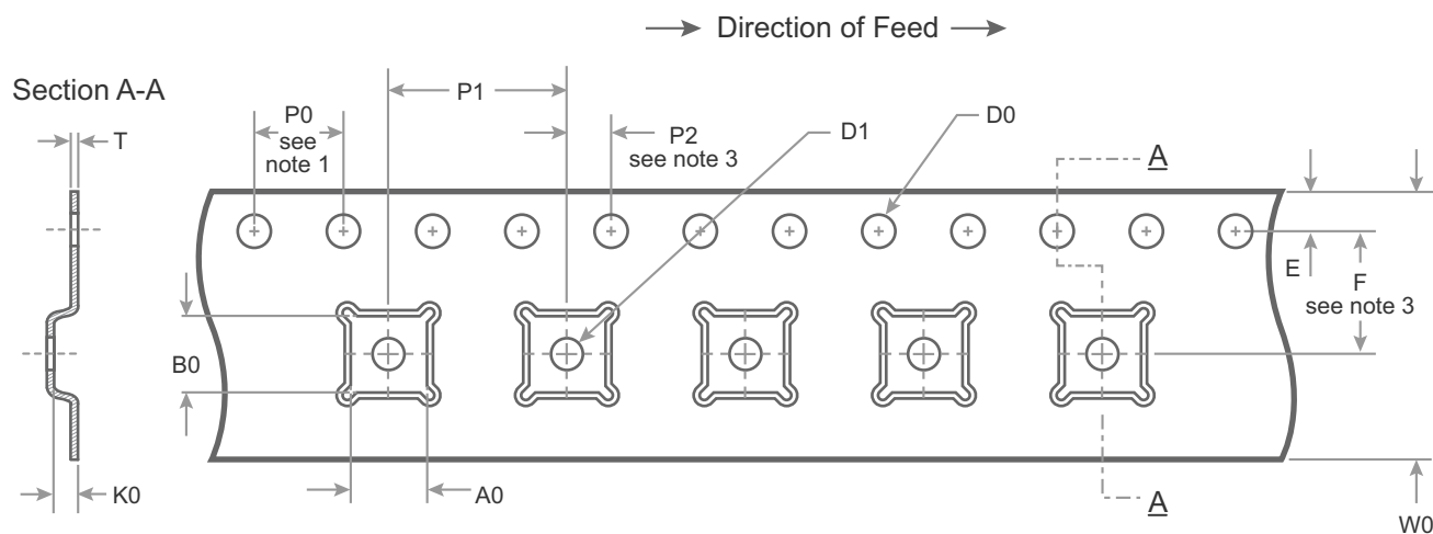
Figure 25 • Tape and Reel Specifications for 32-lead 5 \times 5 \times 0.85 mm QFN
