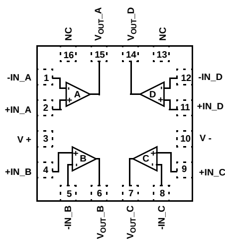
ISL28407 (16 LD QFN) TOP VIEW
