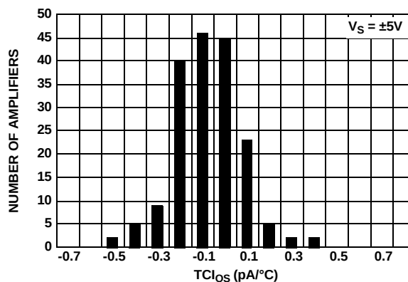
FIGURE 20. TC_{1OS} vs NUMBER OF AMPLIFIERS, V_S = \pm 15V
