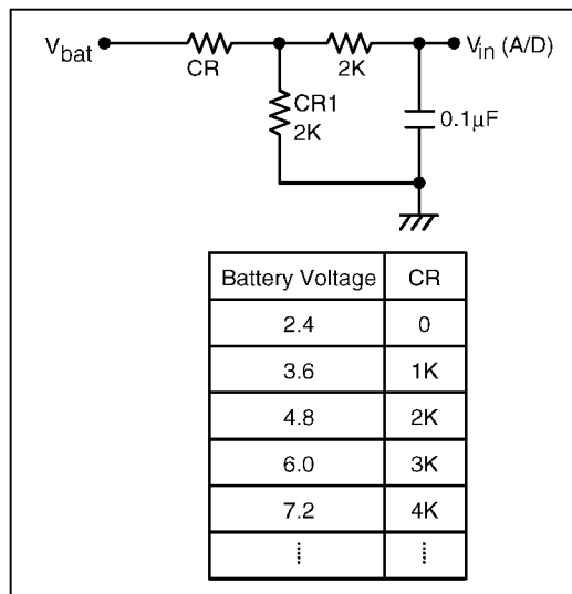
Input RC-Network
