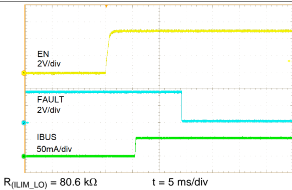
Figure 18. Enable Into Short
