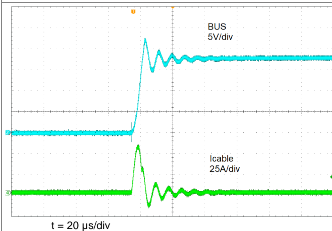
Figure 40. DC-DC VIN Floating, BUS Shorted to Battery
