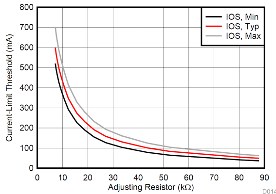
Figure 33. Current-Limit Setting vs Adjusting Resistor
