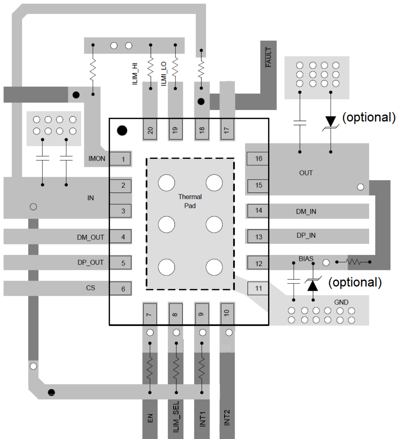
Figure 45. TPD3S713-Q1 Layout Diagram
