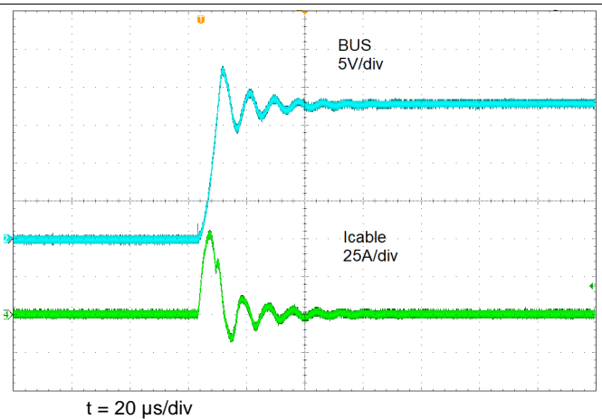
Figure 39. Disabled, 35-V, 1210, X7R C OUT Capacitor With SMAJ18, BUS Shorted to Battery
