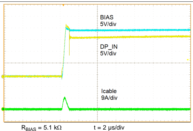
Figure 43. DC-DC VIN Floating, DP_IN Shorted to Battery
