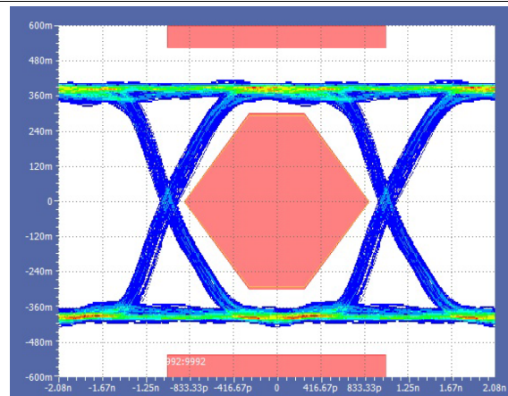
Measured on EVM with 10-cm cable
