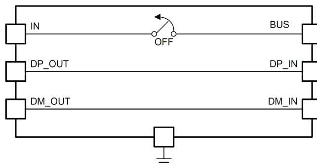
Figure 34. Client-Mode Equivalent Circuit
