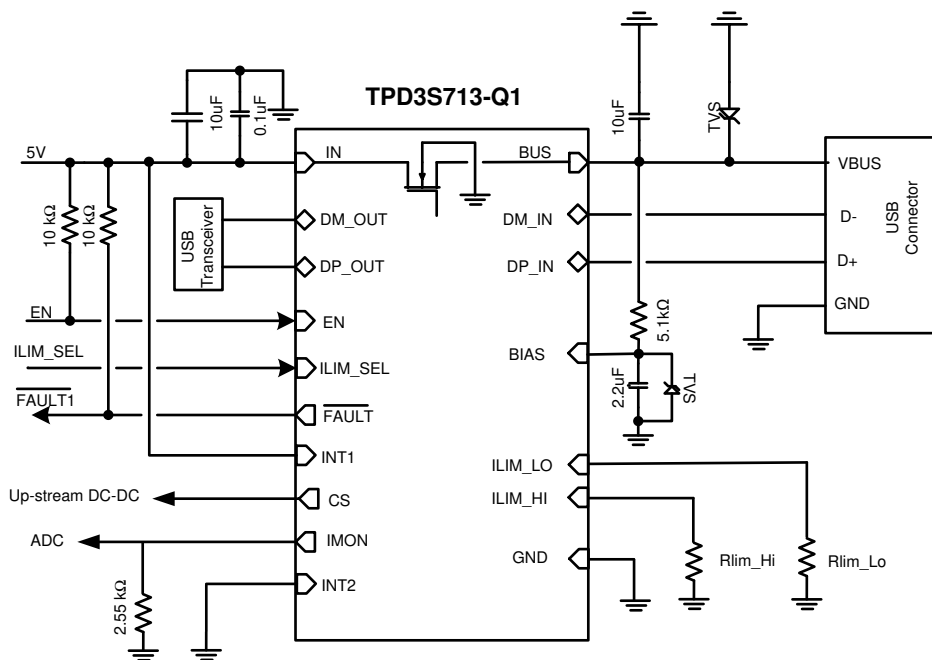
Figure 35. Typical Application Schematic
