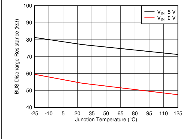
Figure 3. BUS Discharge Resistance (OVP) vs Temperature
