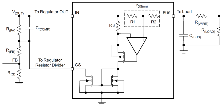
Figure 32. Cable Compensation Equivalent Circuit
