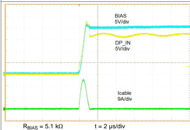
Figure 42. Disabled, DP_IN Shorted to Battery
