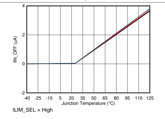
Figure 6. Disabled IN Supply Current vs Temperature
