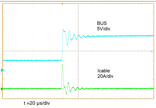
Figure 41. Enable BUS Shorted to Battery
