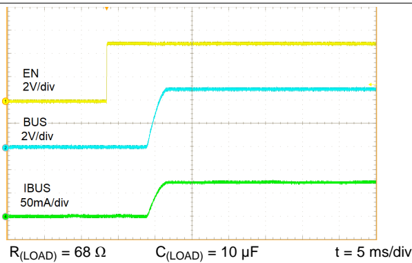
Figure 16. Turnon Response
