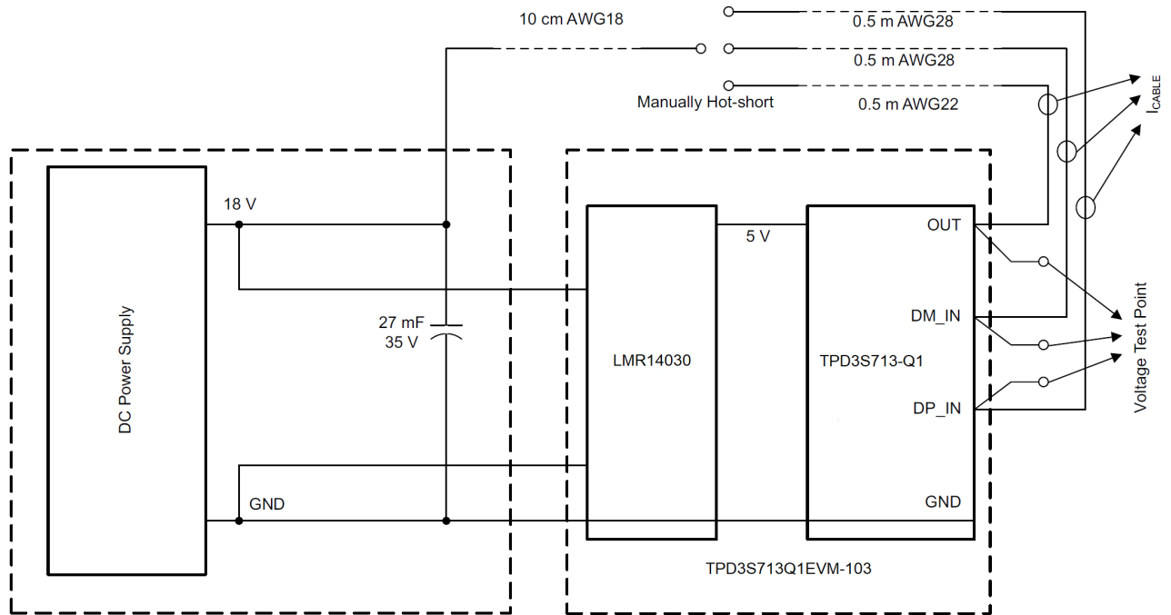
Figure 30. Short-to-Battery System Test Setup
