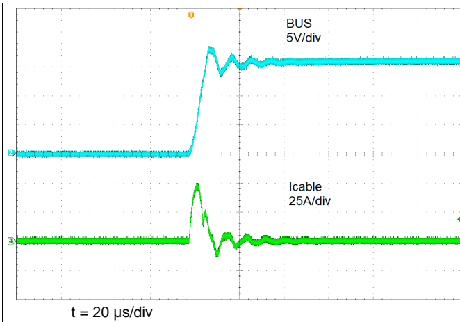
Figure 38. Disabled, 25-V, 1206, X7R C OUT Capacitor With SMAJ16, BUS Shorted to Battery
