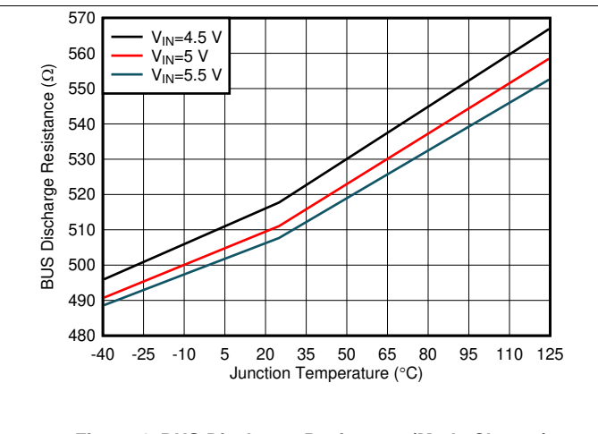
Figure 4. BUS Discharge Resistance (Mode Change) vs Temperature
