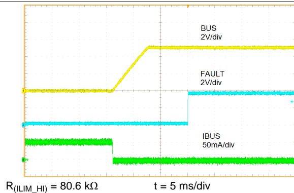
Figure 19. Short Circuit to No Load
