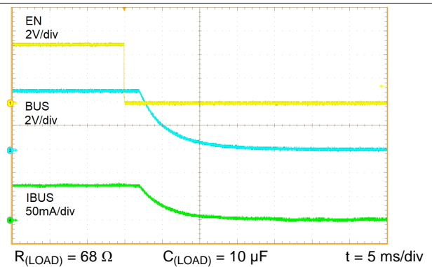
Figure 17. Turnoff Response
