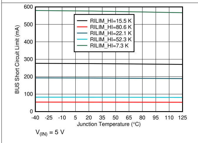
Figure 5. VBUS Short-Circuit Current Limit vs Temperature
