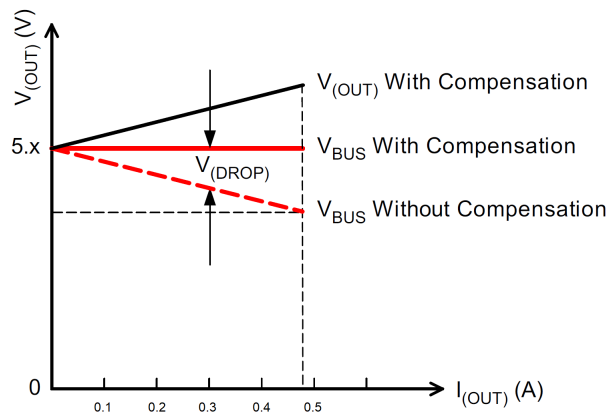
Figure 31. Voltage Drop
