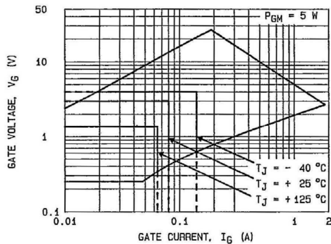
FIG.9 - GATE TRIGGER CHARACTERISTICS.
