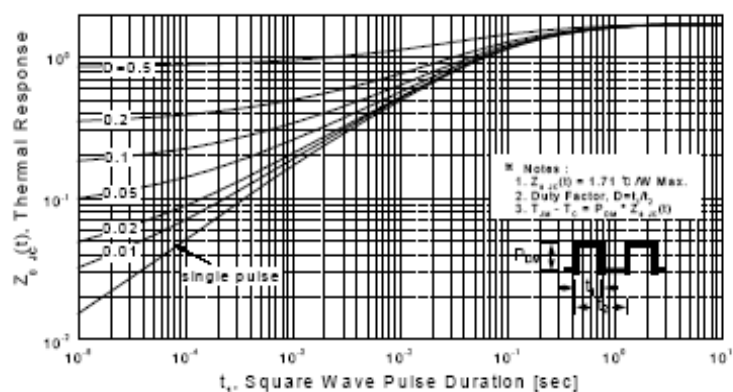
Figure 11-1. Transient Thermal Response Curve for HM730
