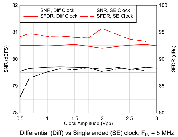
Figure 6-52. AC Performance vs Clock Amplitude
