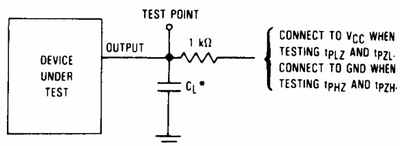
Figure 4. Test Circuit
