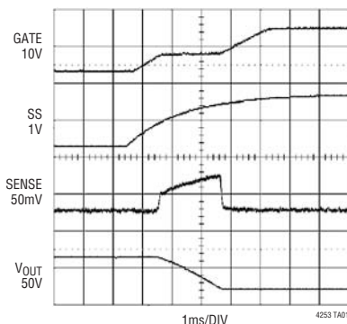
Start-Up Behavior
