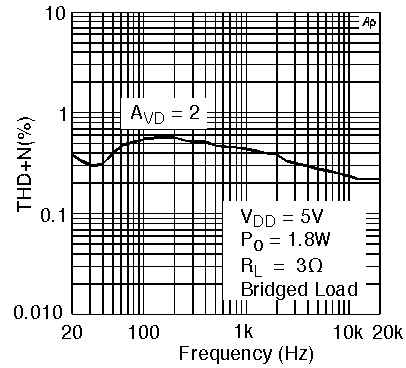
LM4867MTE THD+N vs Frequency
