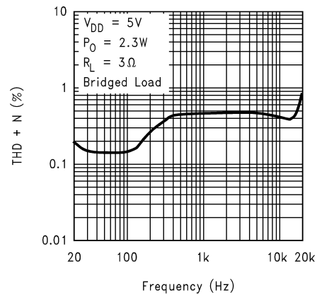
LM4867LQ THD+N vs Frequency
