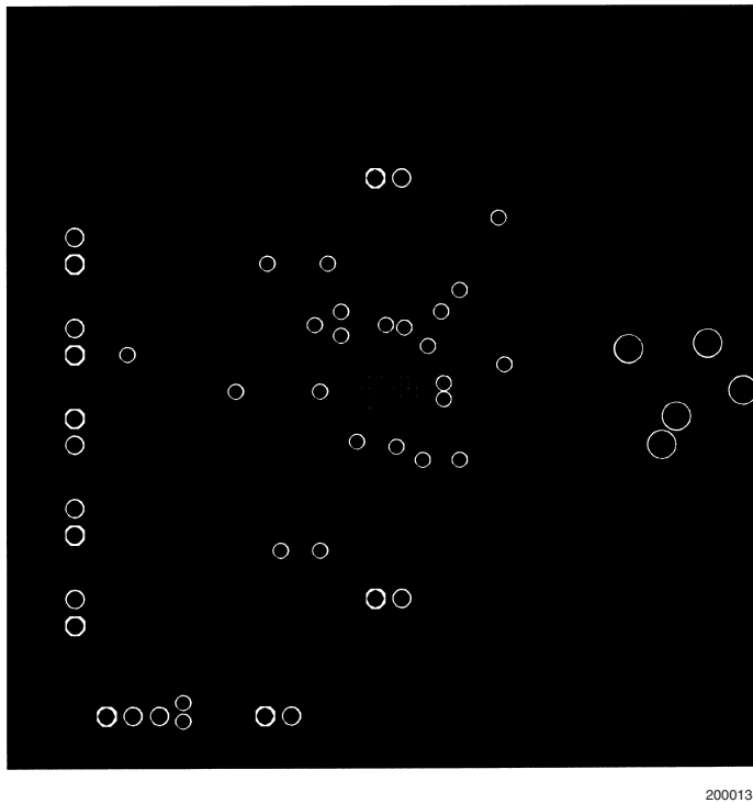
FIGURE 16. Recommended MTE PC Board Layout: Upper Inner-Layer Layout
