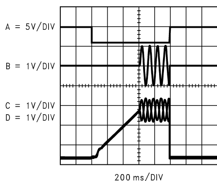
FIGURE 2. Differential output signal (Trace B) is devoid of transients. The SHUTDOWN pin is driven by a shutdown signal (Trace A). The inverting output (Trace C) and the non-inverting output (Trace D) are applied across an 8\Omega BTL load.
