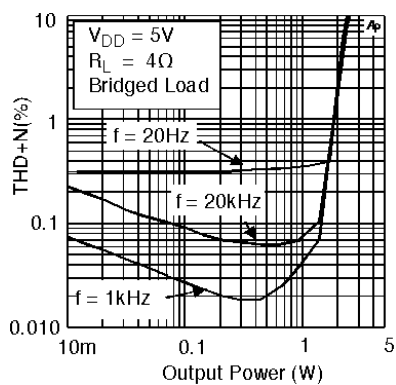
LM4867MTE THD+N vs Output Power
