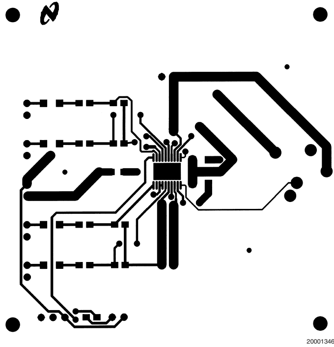
FIGURE 15. Recommended MTE PC Board Layout: Component-Side Layout
