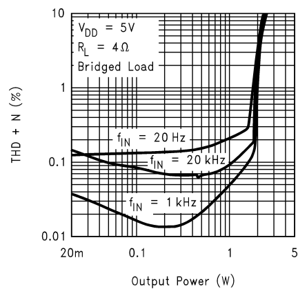
LM4867LQ THD+N vs Output Power
