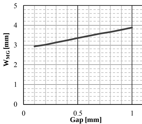
Magnetic detection width vs. gap
