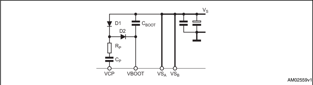
Figure 8. Charge pump circuit
