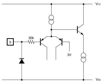
SCL (5pin)
