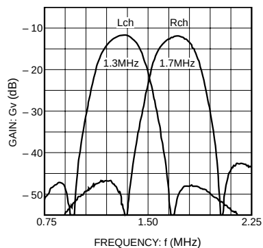
Fig. 3 FM BPF frequency characteristics (NTSC)
