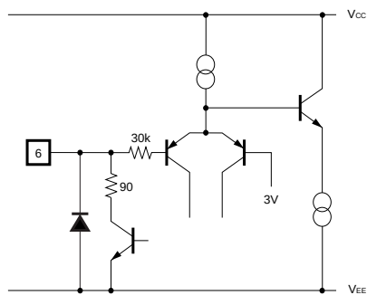
SDA (6pin)
