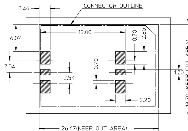
RECOMMENDED PCB LAYOUT(±0.05MM)
