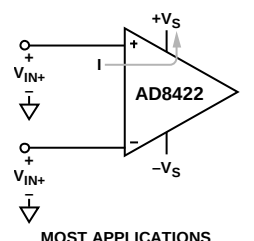
Figure 60. Input Overvoltage Protection with no External Components
