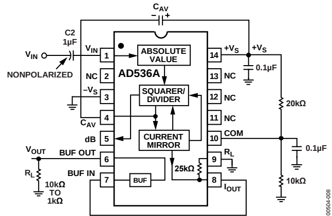
Figure 17. Single-Supply Connection
