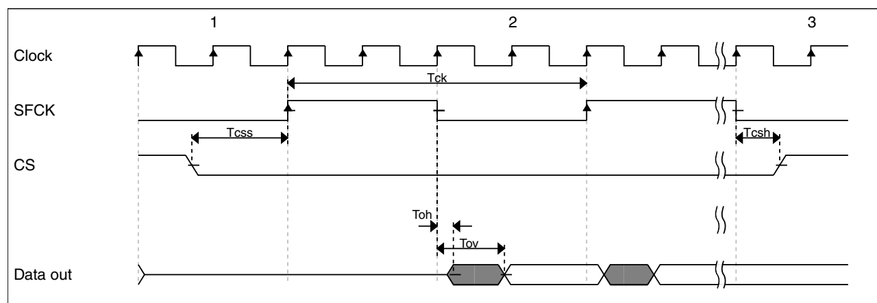
Figure 12. QuadSPI output timing (SDR mode) diagram
