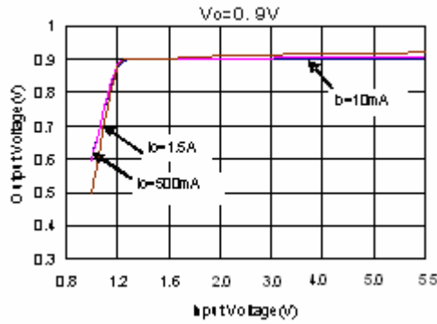
1. Output Voltage vs Input Voltage
