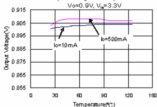
3. Output Voltage vs Temperature
