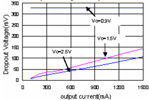
8. Dropout Voltage vs Output Current
