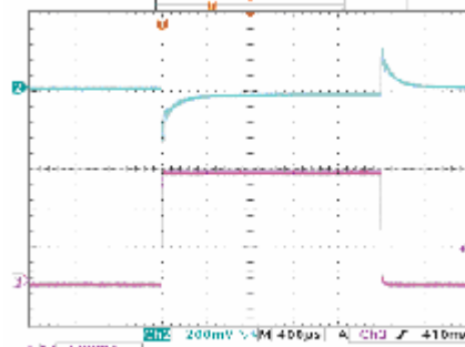
10. Load Transient Response
