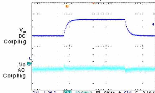
11. Line Transient Response
