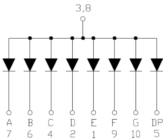
Common Anode
