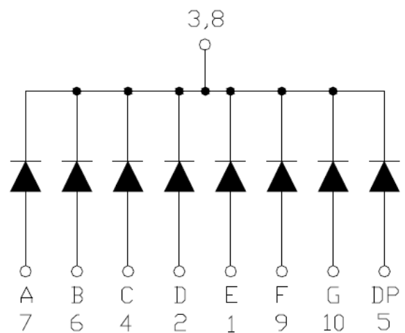
Common Cathode
