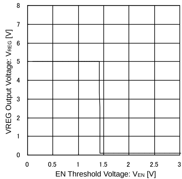
Figure 11. VREG Output Voltage vs EN Threshold Voltage
