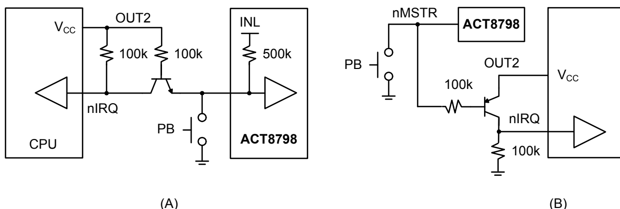
Figure 2: Simple Circuits
