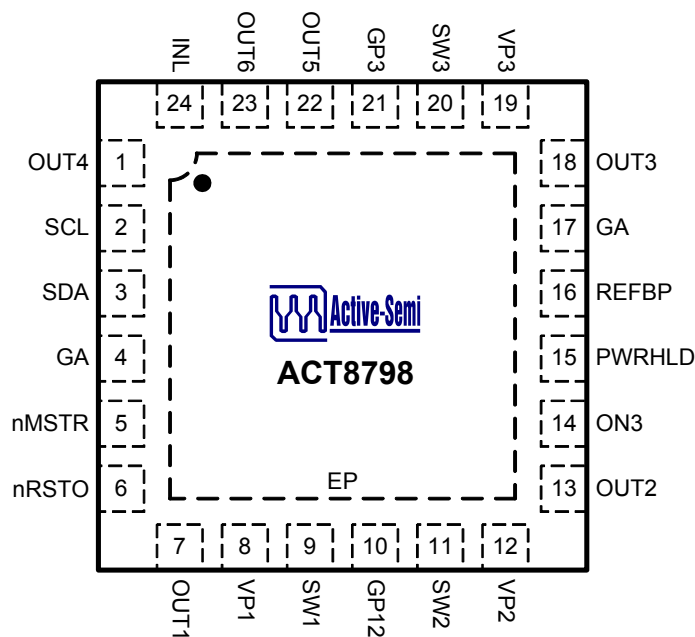
Thin - QFN (TQFN44-24)
