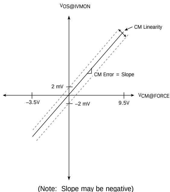
Figure 2. Graphical Representation of Common Mode Error
