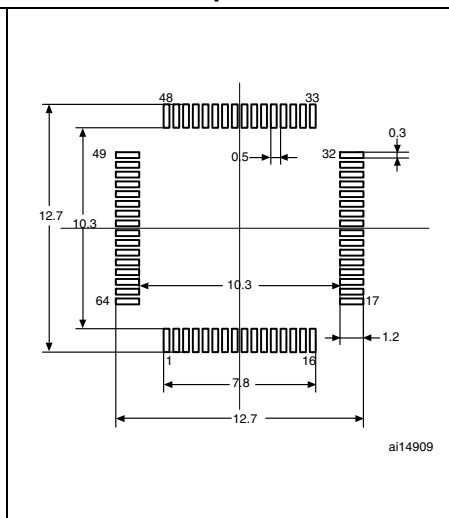
Figure 42. Recommended footprint (1)(2)
