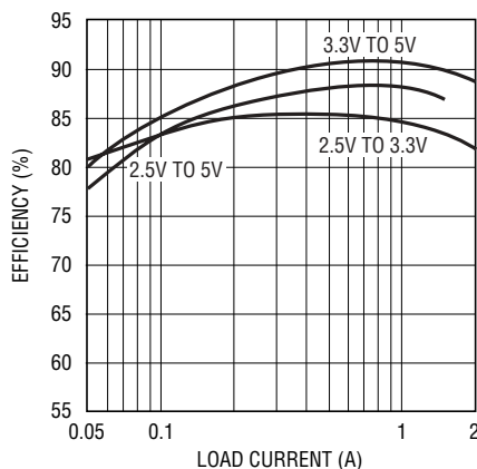
Converter Efficiency
