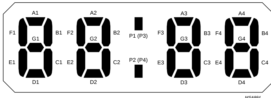
Fig.2 Segment designation of LCD.
