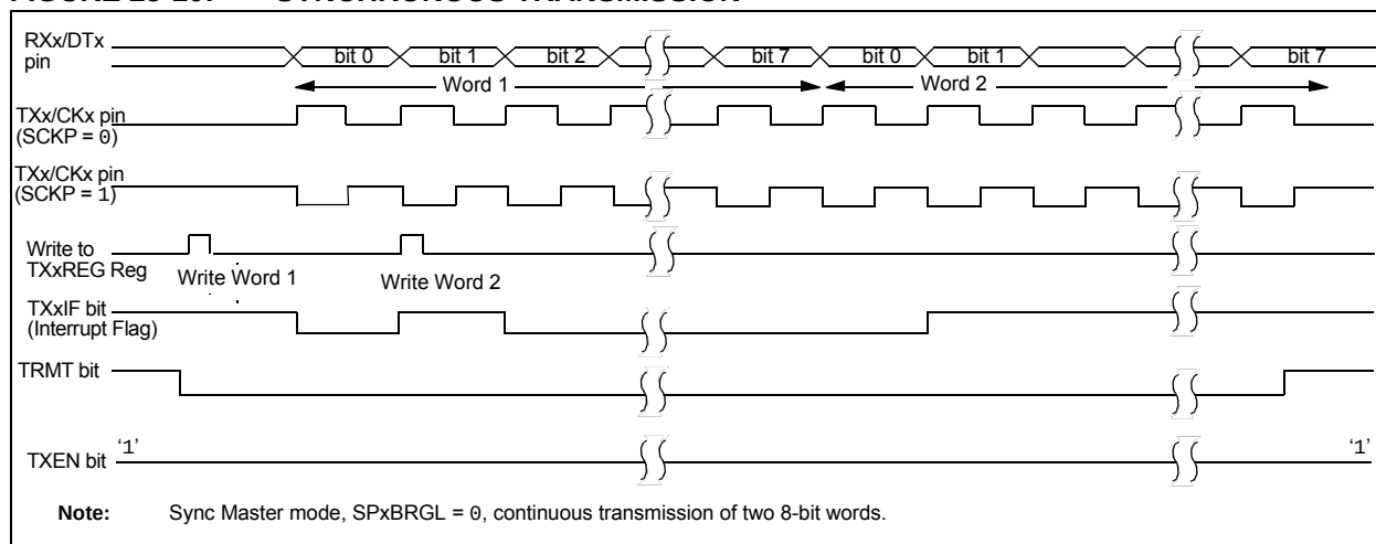
FIGURE 25-10: SYNCHRONOUS TRANSMISSION
