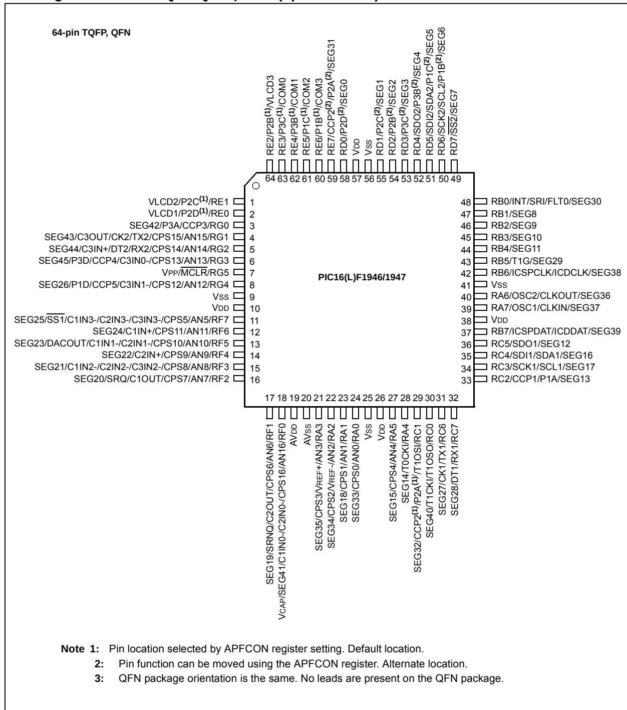
Pin Diagram – 64-Pin TQFP/QFN (PIC16(L)F1946/1947)
