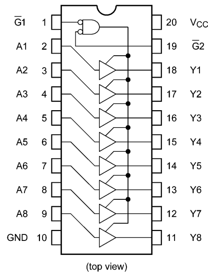
74HCT541D
