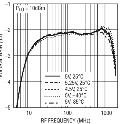
Voltage Gain vs RF Frequency ( P_{LO} = 10dBm )
