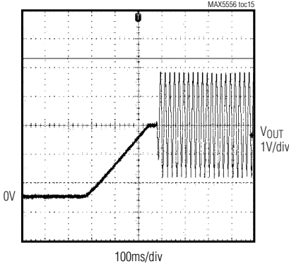
POWER-UP RESPONSE
