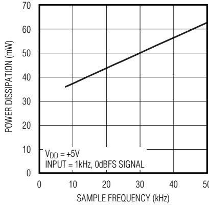
POWER DISSIPATION vs. SAMPLE FREQUENCY
