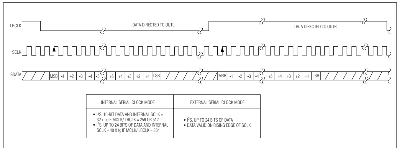
Figure 4. MAX5556 Data Format Timing
