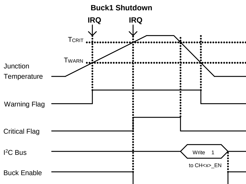
Figure 4: Temperature Protection Operation
