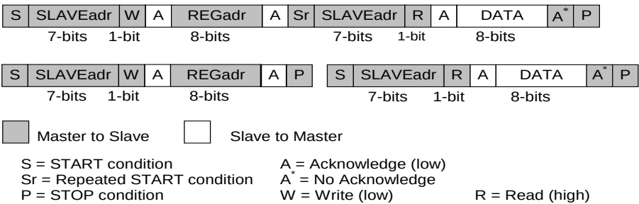
Figure 8: I²C Byte Read (SDA Line) Examples
