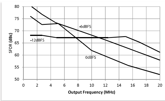
Figure 20c. SFDR vs fout, fclk = 50MHz
