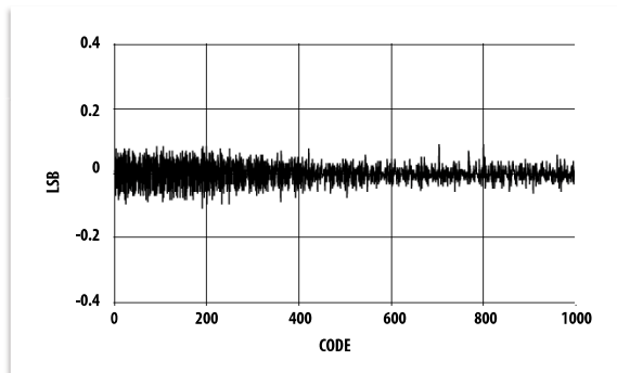
Figure 17. Differential Nonlinearity
