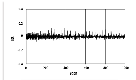
Figure 29. Differential Nonlinearity
