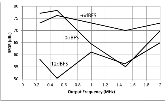
Figure 20a. SFDR vs fout, fclk = 5MHz
