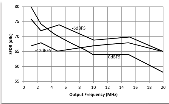
Figure 7c. SFDR vs fout, fclk = 50MHz
