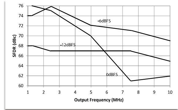
Figure 7b. SFDR vs fout, fclk = 25MHz
