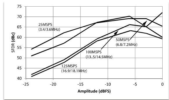
Figure 19b. SFDR vs Amplitude, fclk = 10 x fout
