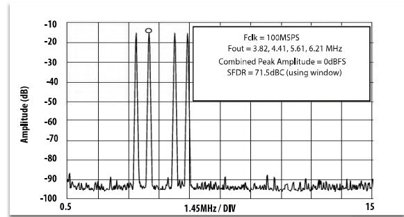
Figure 14. SFDR Four Tones, fclk = 100MHz
