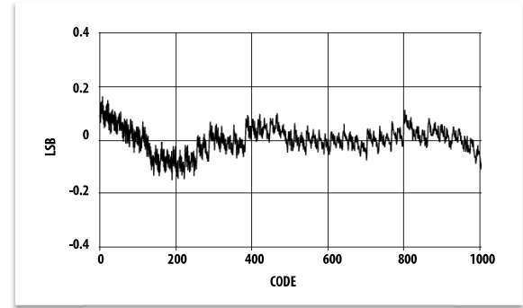
Figure 16. Integral Nonlinearity
