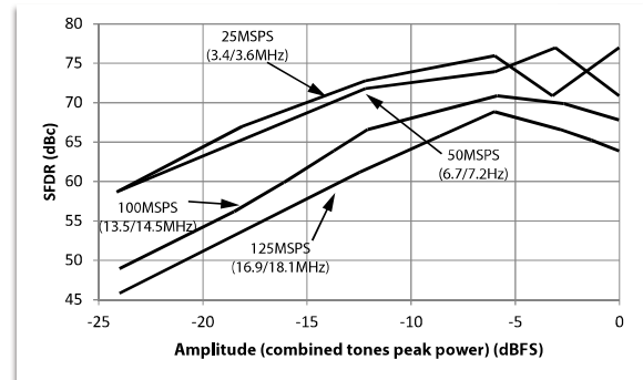
Figure 8. SFDR vs Amplitude of Two Tones, f_{clk} = 7 \times f_{out}
