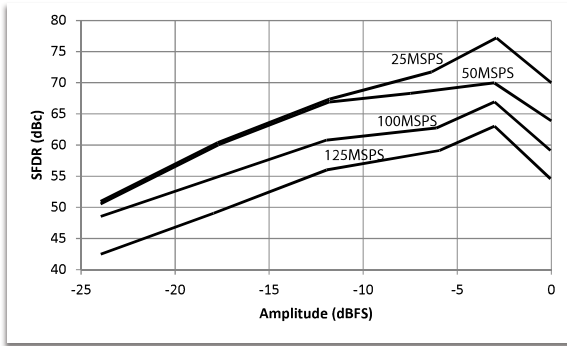
Figure 6b. SFDR vs Amplitude, fclk = 5 x fout
