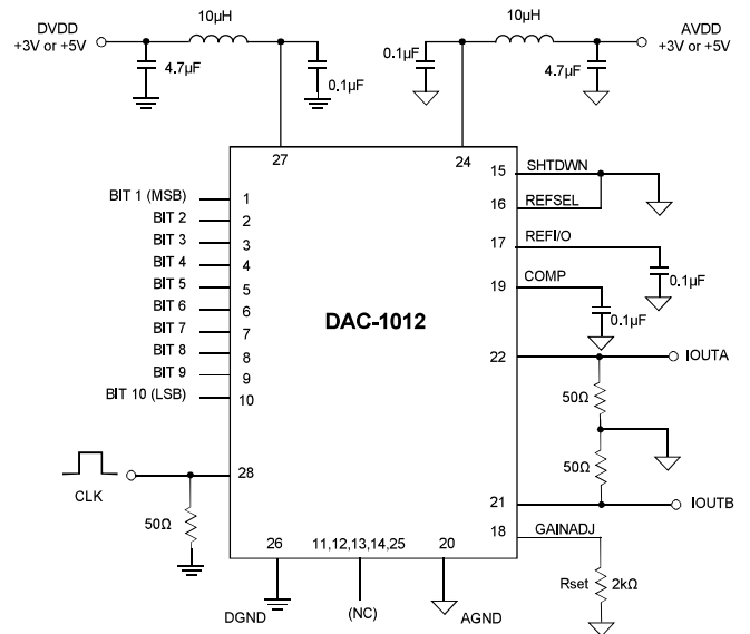
Figure 3. Typical Connection Diagram
