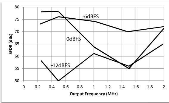
Figure 7a. SFDR vs fout, fclk = 5MHz
