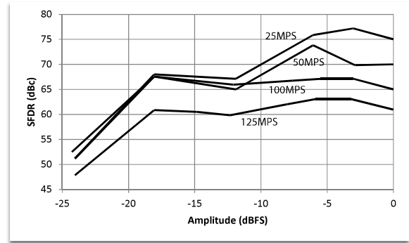
Figure 6a. SFDR vs Amplitude, fclk = 10 x fout
