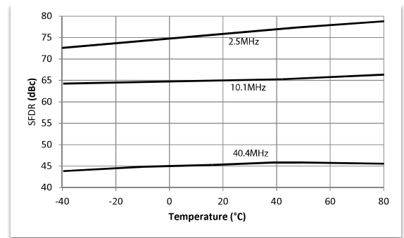
Figure 23. SFDR vs Temperature, fclk = 100MHz
