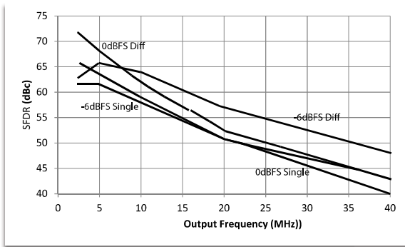
Figure 22. Differential vs Single-ended, fclk = 100MHz
