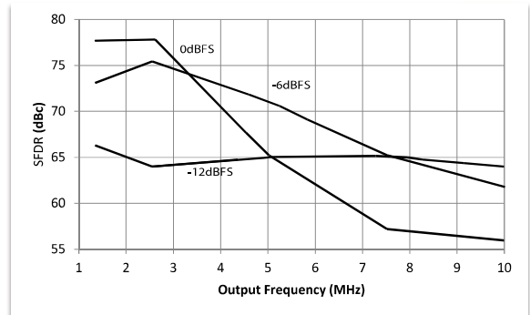
Figure 20b. SFDR vs fout, fclk = 25MHz
