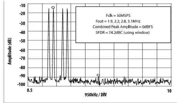
Figure 27. SFDR Four Tones, fclk = 50MHz
