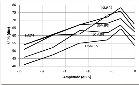
Figure 19a. SFDR vs Amplitude, fclk = 5 x fout
