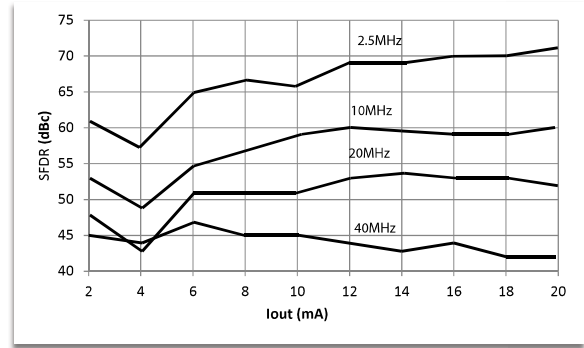
Figure 21. SFDR vs Iout, fclk = 100MHz
