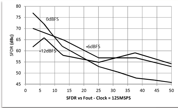
Figure 20e. SFDR vs fout, fclk = 125MHz
