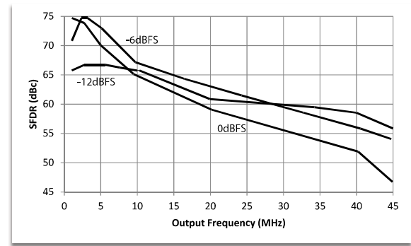
Figure 7d. SFDR vs fout, fclk = 100MHz
