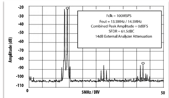
Figure 25. SFDR Two Tone, fclk = 100MHz
