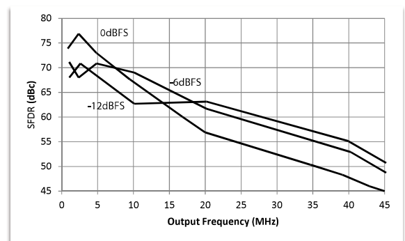
Figure 20d. SFDR vs fout, fclk = 100MHz
