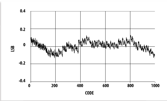
Figure 28. Integral Nonlinearity
