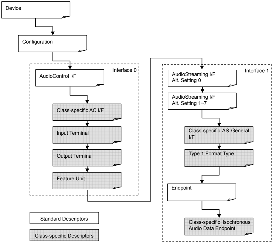
Figure 20. Descriptor Hierarchy
