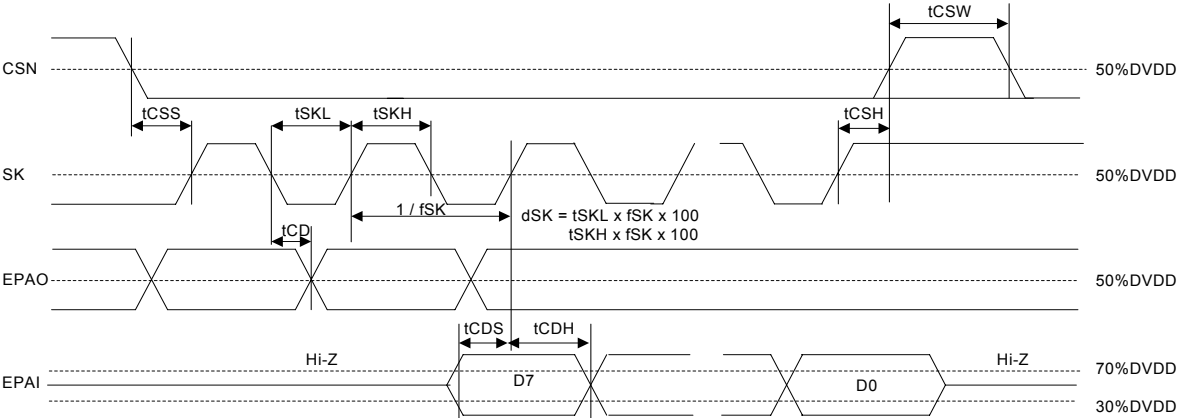
Figure 11. SPI (EEP-ROM) Control Interface Timing
